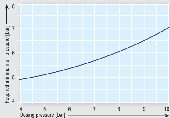
PRESSURE DIAGRAM
